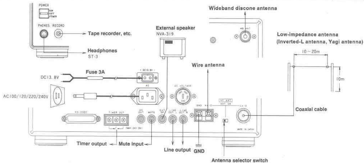
Figure 3-6 How to Connect the External Terminals
