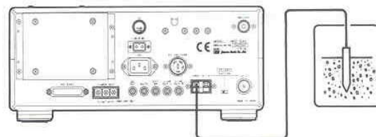
Figure 3-4 Connecting the Earth
